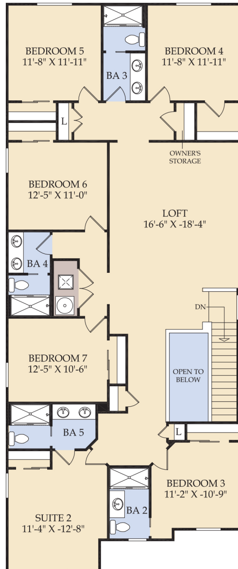
Second Floor
