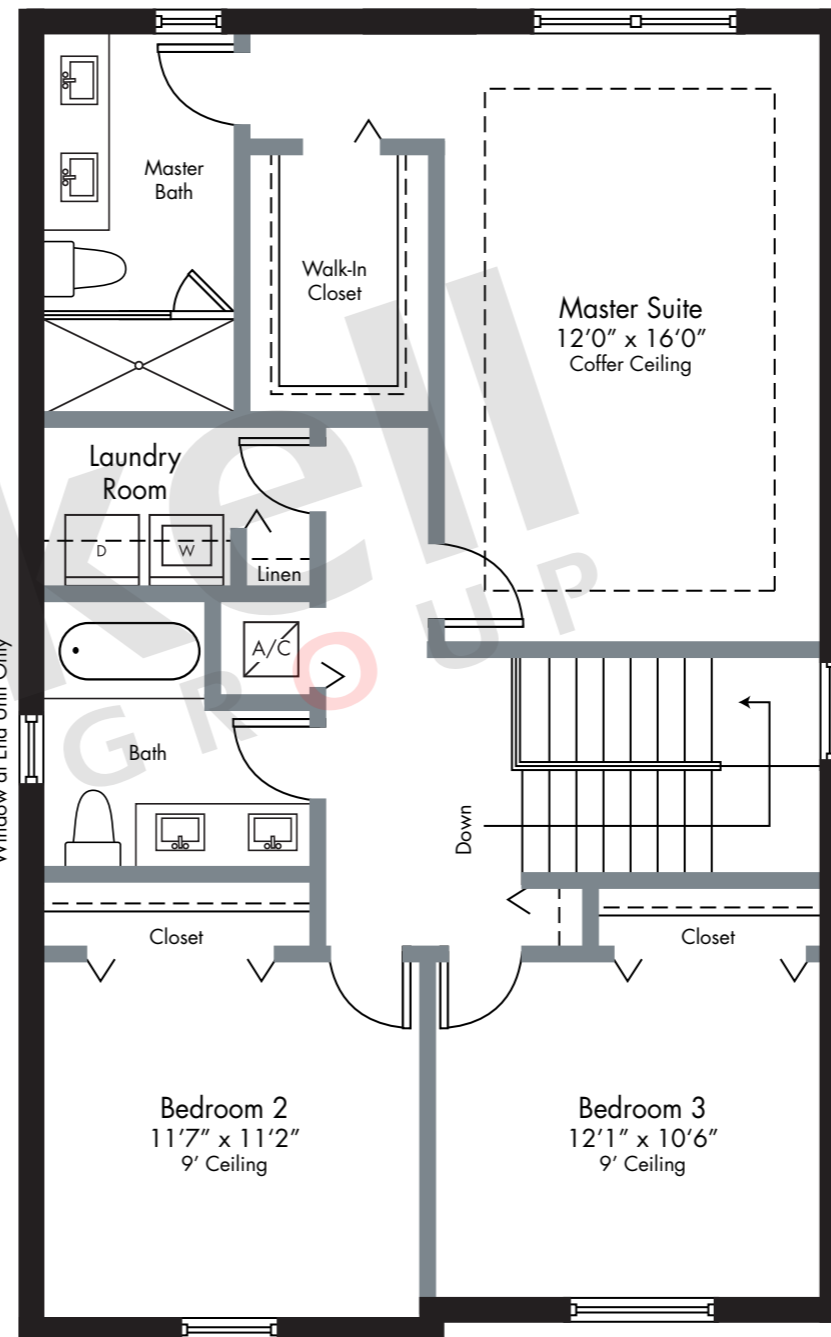
Second Floor
