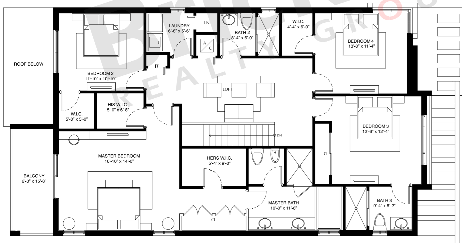
SECOND FLOOR
