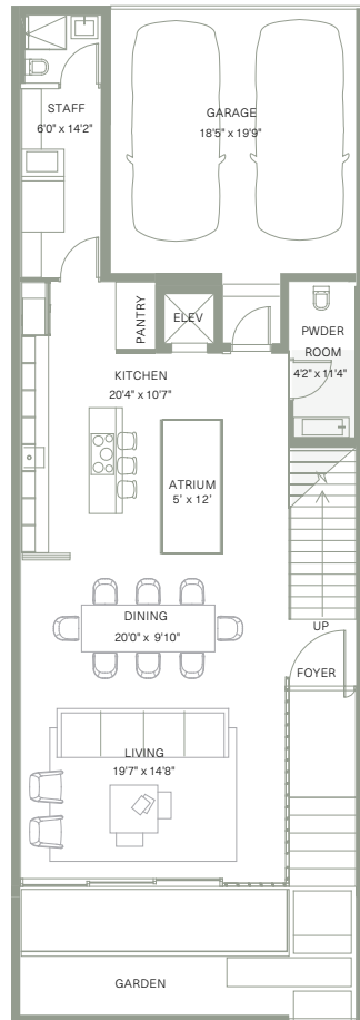
FIRST FLOOR
