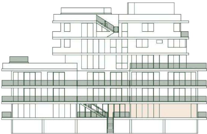
EAST FACADE
