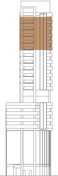
EAST ELEVATION
