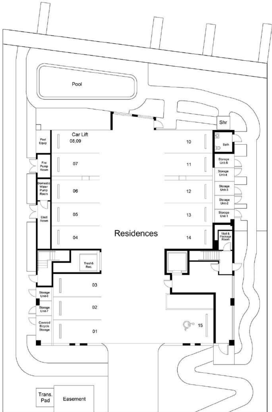
FIRST FLOOR
