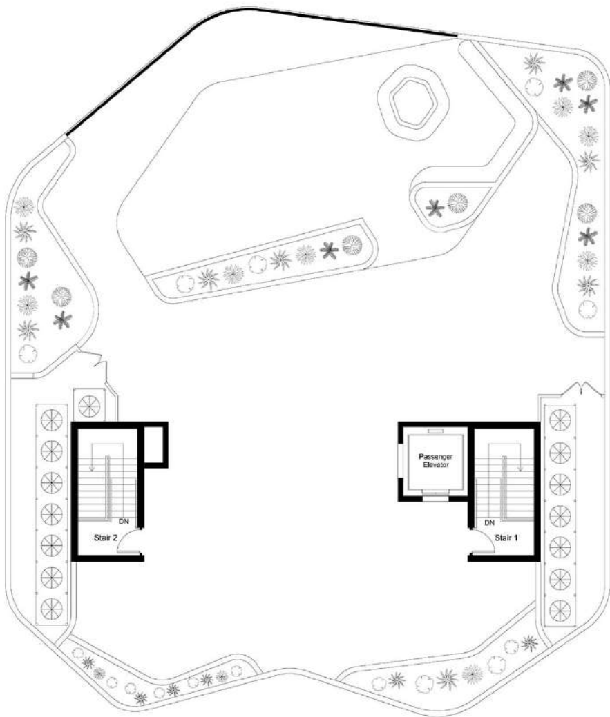
ROOF PLAN
